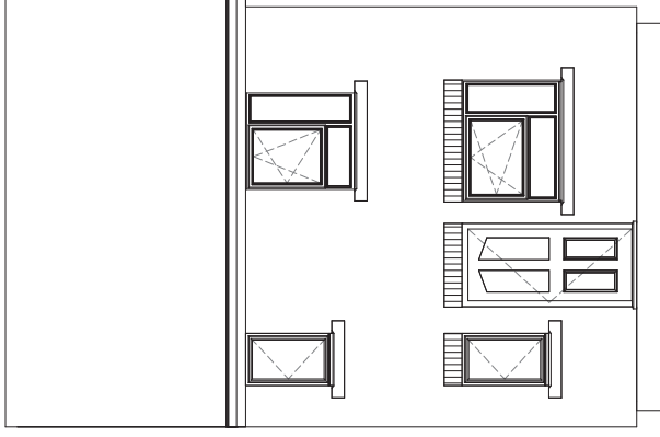
2 Rear Elevation 1 : 50
